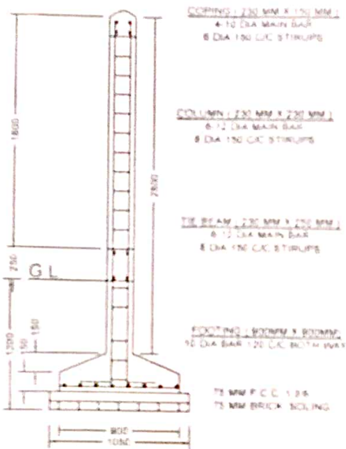
COLUMN CROSS SECTION COLUMN INTERVAL 2400 MM
